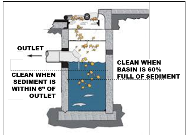
Remove sediment from a catch basin if it fills 60% of the sump or comes within 6" of a pipe.
